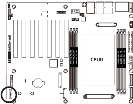
USB 3.0 Connector
