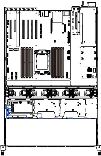
SAS Expander Card to HDD Back Panel Board Cable #1
