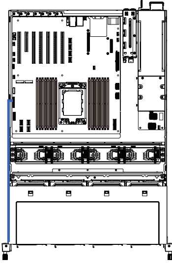
HDD Back Plane Board Power Cable
