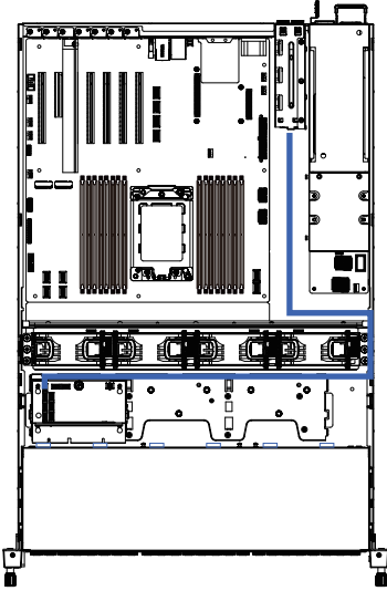
SAS Expander Card to HDD Back Panel Board Cable #1
