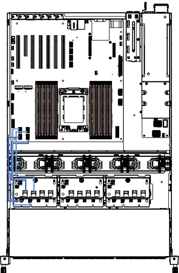
NVMe Expander Card Cable #0-#3
