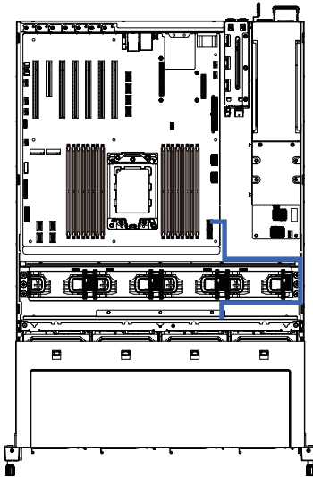
On-Board SATA to HDD Back Panel Board HBA Cable Cable
