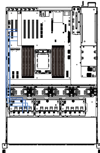
NVMe Expander Card Cable #4-#7
