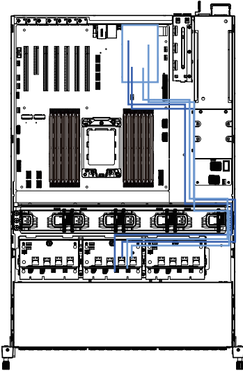
NVMe Expander Card Cable #12-#15
