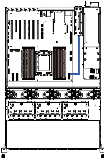
Rear HDD Back Panel Board SATA Cable
