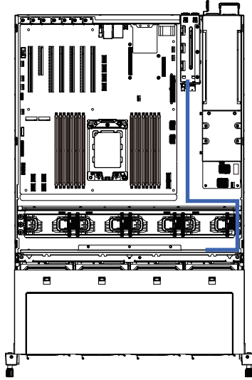
SAS Expander Card to HDD Back Panel Board Cable #2
