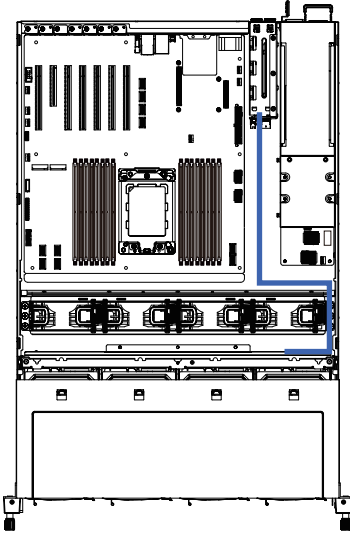
Rear HDD Back Panel Board Signal Cable
