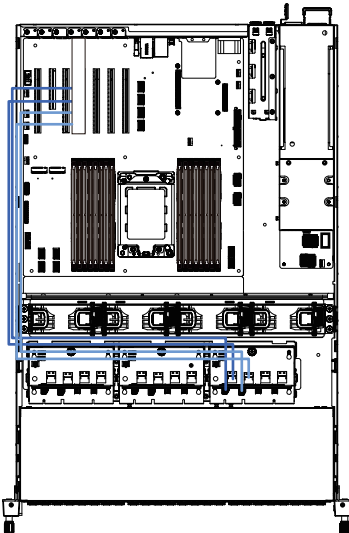
NVMe Expander Card Cable #16-#19
