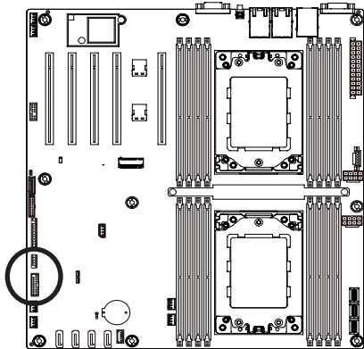
USB 2.0 Header
