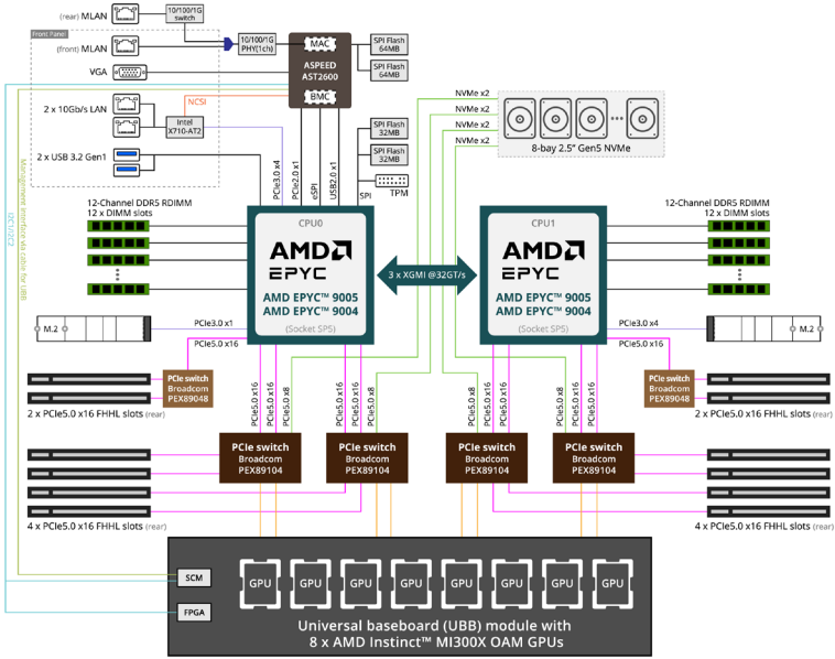
G893-ZX1-AAX2 System Block Diagram
