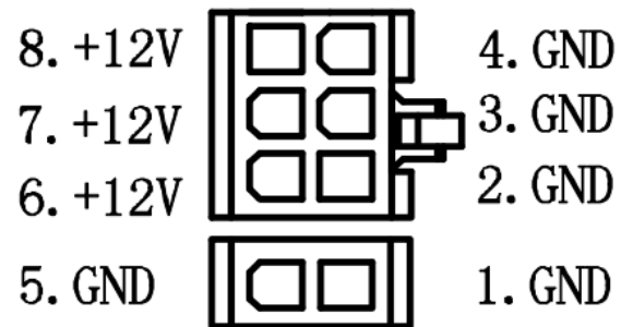
PCI-E 6+2 pin VGA Side
