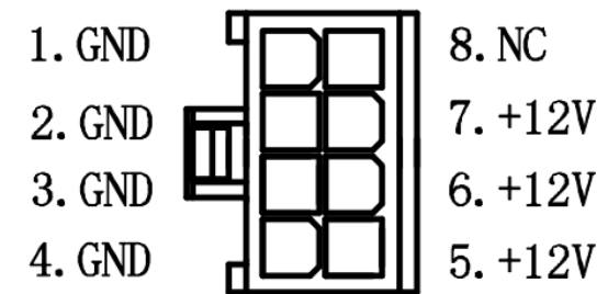
PCI-E 6+2 pin PSU Side
