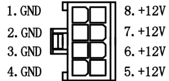
CPU 4+4 pin PSU Side
