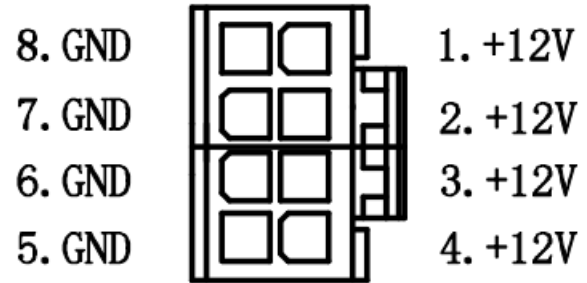
CPU 4+4 pin M/B Side
