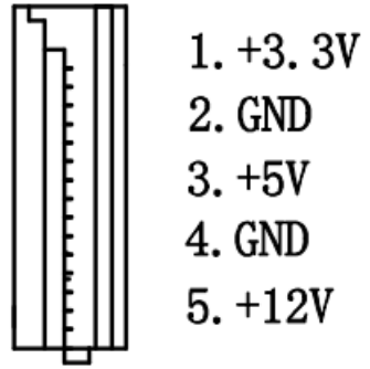
SATA & PATA Component Side
