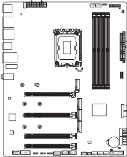
12V_2X4_1 12V_2X4_2
