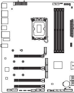
12V_2X4_1, 12V_2X4_2
