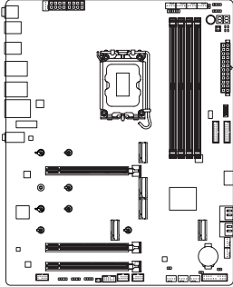
12V_2X4_1
