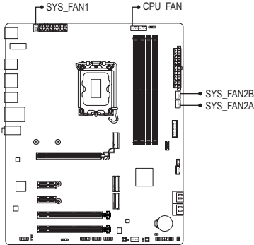
SYS_FAN1/SYS_FAN2A/2B
