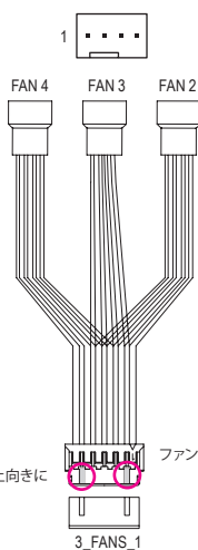
SYS_FAN2/3/4:
