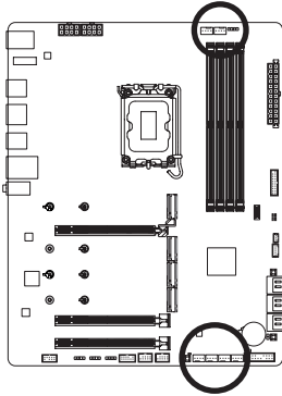
CPU_FAN 1 SYS_FAN1/SYS_FAN2/ SYS_FAN3
