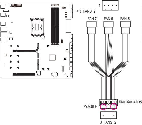
SYS_FAN5/6/7_PUMP:
