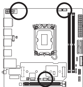
CPU_FAN
