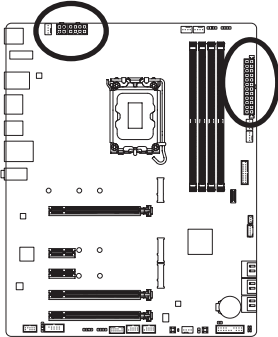
ATX_12V_2X4:
