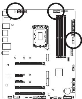
SYS_FAN1/SYS_FAN2A/2B
