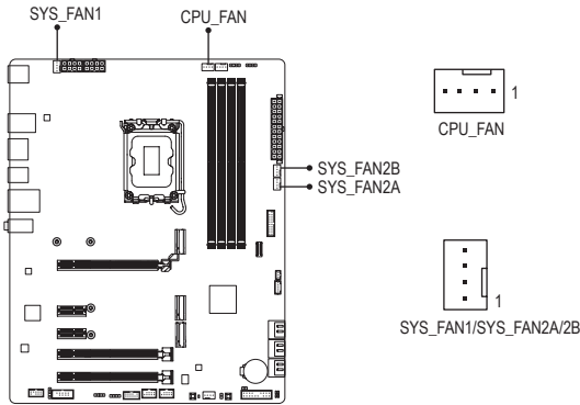
CPU_FAN/SYS_FAN1/2A:
