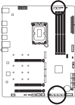
1 CPU_FAN 1 SYS_FAN1/SYS_FAN2/ SYS_FAN3
