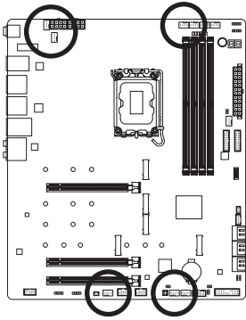
SYS_FAN1/SYS_FAN2
