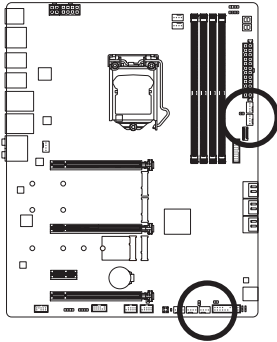
SYS_FAN5_PUMP
