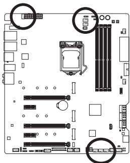
SYS_FAN2/3/4
