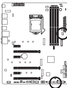
SYS_FAN5_PUMP
