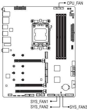
CPU_FAN 1 SYS_FAN1/SYS_FAN2/SYS_FAN3
