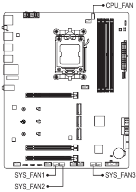
SYS_FAN1/2/3
