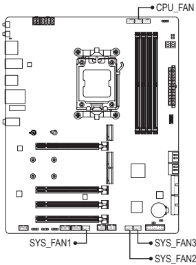
SYS_FAN1/2/3
