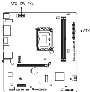
ATX_12V_2X4:
