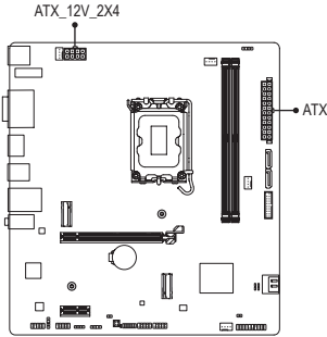
ATX_12V_2X4:
