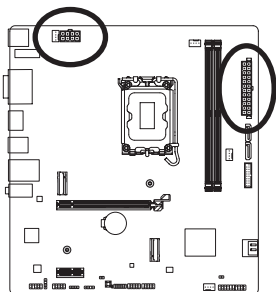
ATX_12V_2X4:
