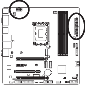
ATX_12V_2X4:
