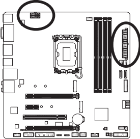
ATX_12V_2X4:
