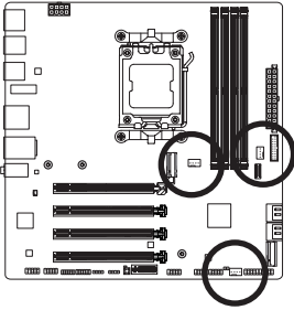
CPU_FAN/SYS_FAN1
