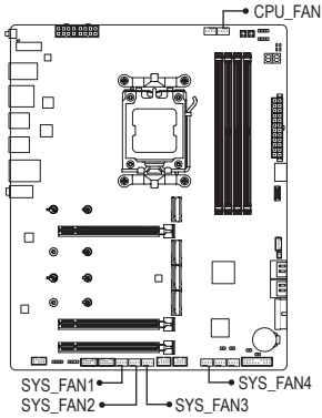
1 CPU_FAN 1 SYS_FAN1/SYS_FAN2/ SYS_FAN3/SYS_FAN4
