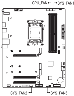
CPU_FAN/SYS_FAN1
