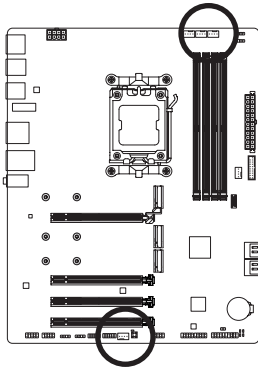
CPU_FAN/SYS_FAN1
