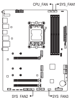
CPU_FAN/SYS_FAN1
