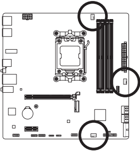
CPU_FAN/SYS_FAN2
