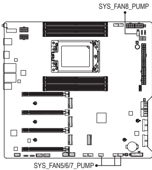
SYS_FAN5/6/7_PUMP
