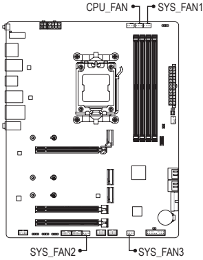
CPU_FAN/SYS_FAN1
